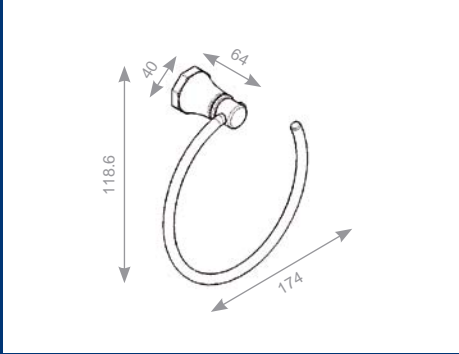
Towel Ring
