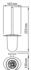
Toilet Brush Holder 113171
